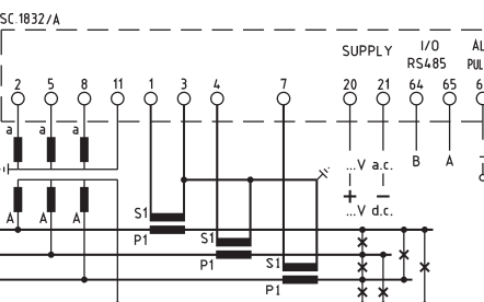
Q72P3H005MCQ...O per linea trifase 4 fili / for three-phase four wires system
