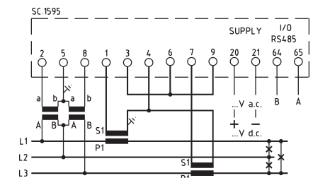
Q72P3H005MCQ... per linea trifase 3 fili / for three-phase three wires system
