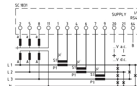
Q72P3H005MCQ... per linea trifase 4 fili / for three-phase four wires system
