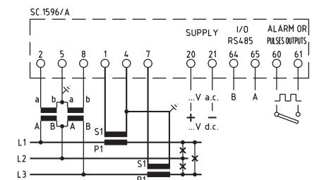
Q72P3H005MCQ...O per linea trifase 3 fili / for three-phase three wires system
