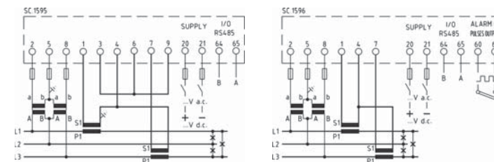
Q52P3H005MCQ... per linea trifase 3 fili / for three-phase three wires system
