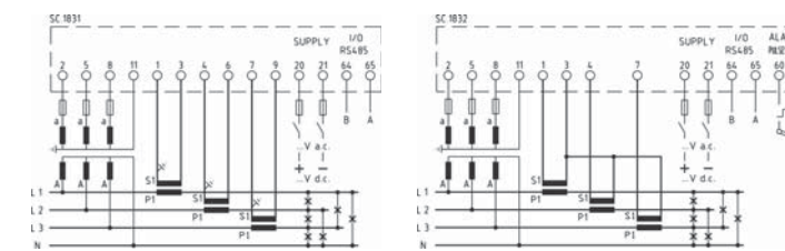
Q52P3H005MCQ... per linea trifase 4 fili / for three-phase four wires system
