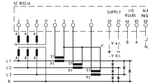
Q72P3H005MCQ...O per linea trifase 4 fili / for three-phase four wires system
