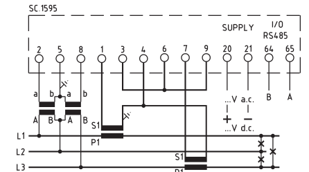
Q72P3H005MCQ... per linea trifase 3 fili / for three-phase three wires system
