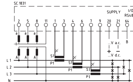
Q72P3H005MCQ... per linea trifase 4 fili / for three-phase four wires system
