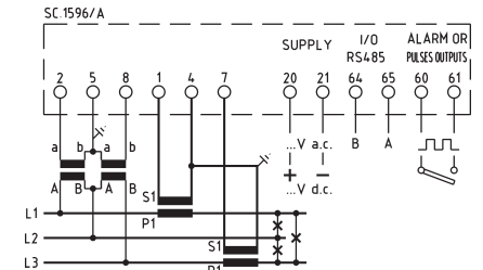
Q72P3H005MCQ...O per linea trifase 3 fili / for three-phase three wires system
